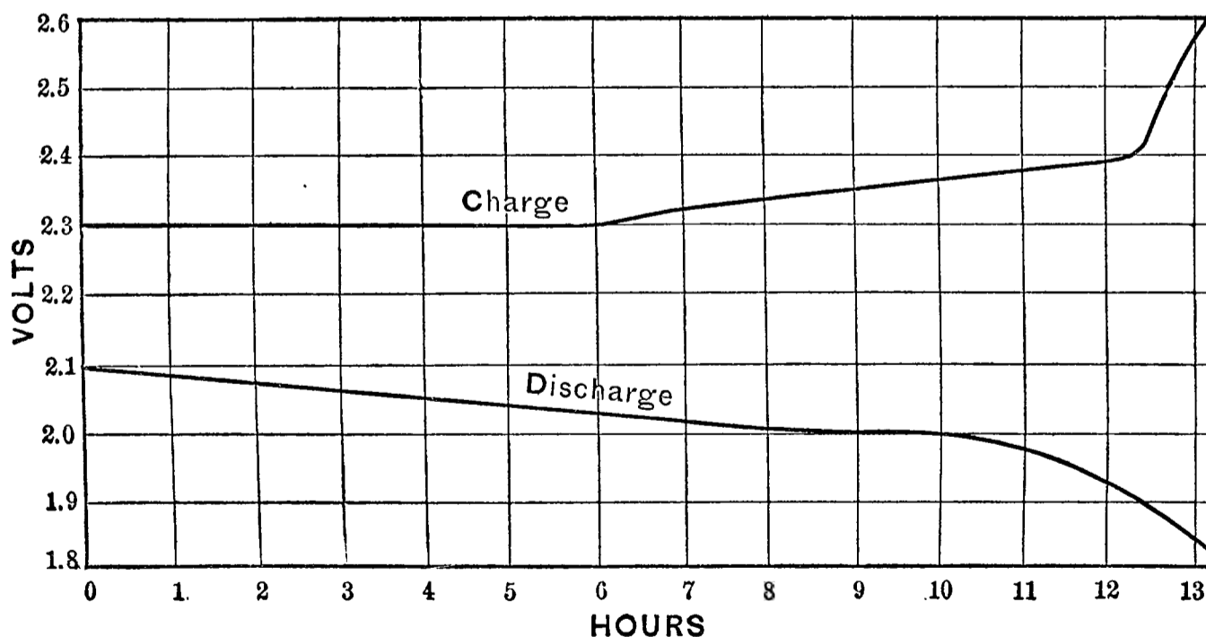
Discharge Curve of Bradbury-Stone Battery. Class B 2, (3).
